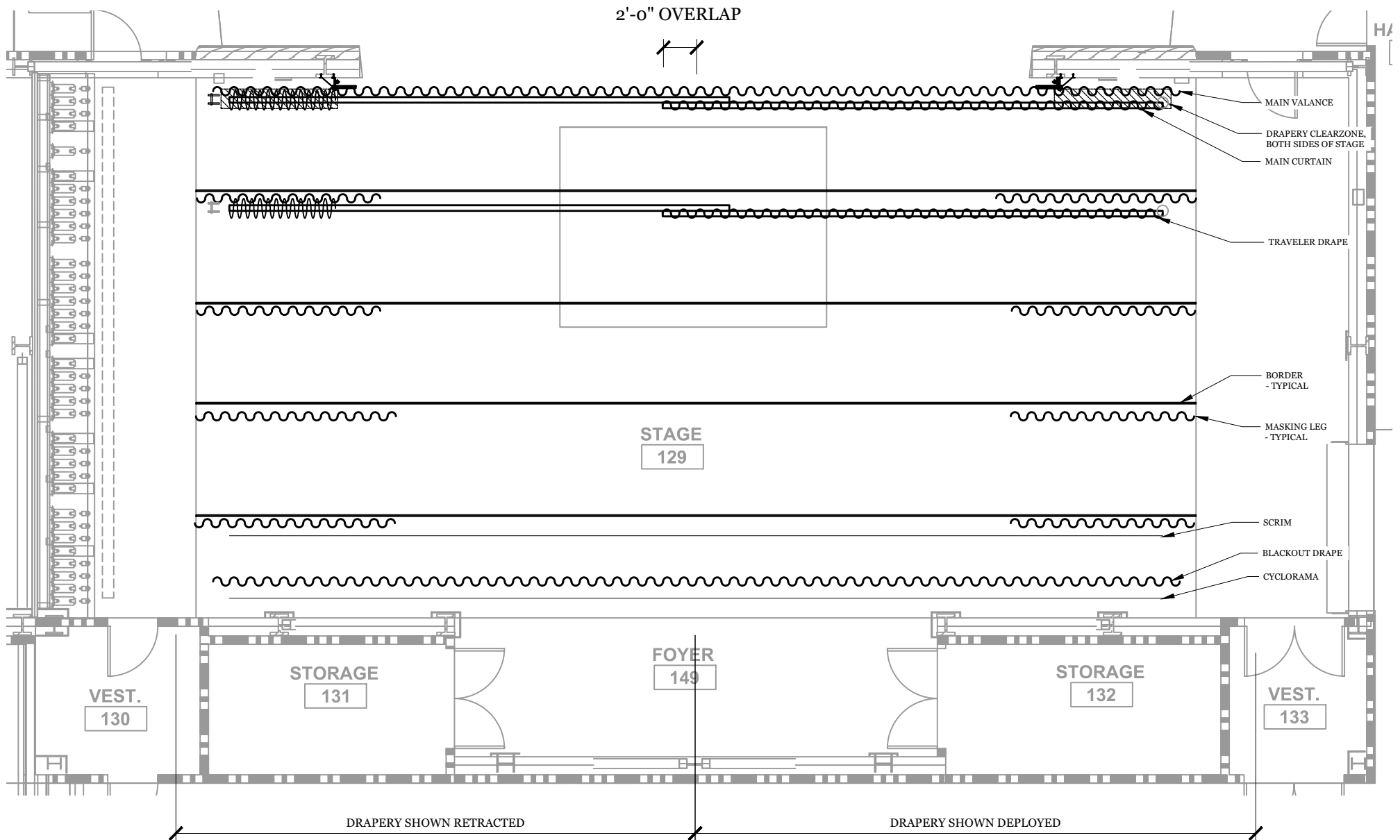
1 MAIN THEATRE - PLAN AT STAGE LEVEL 1/8" = 1'-0"
