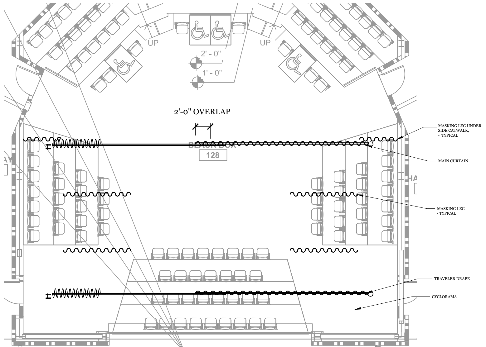
1 BLACK BOX THEATRE - PLAN AT STAGE LEVEL 1/8" = 1'-0"
